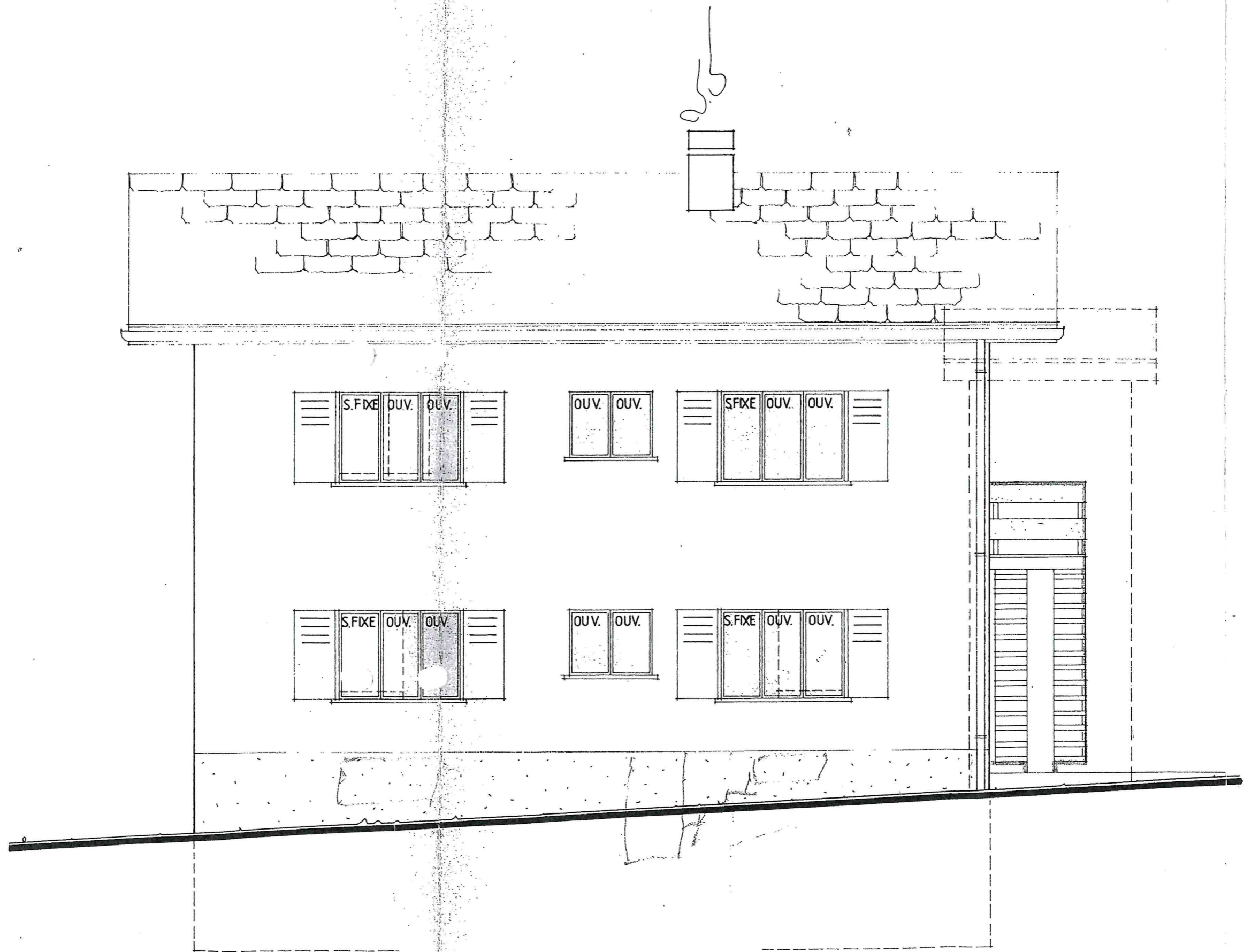
FACADE SUD
